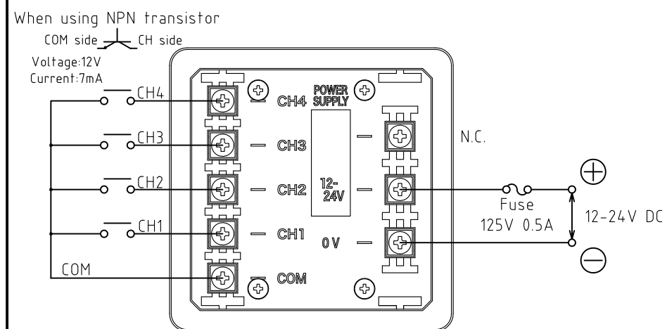
■ BD-24A Wiring diagram
